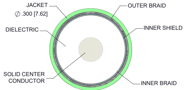
SECTION VIEW
