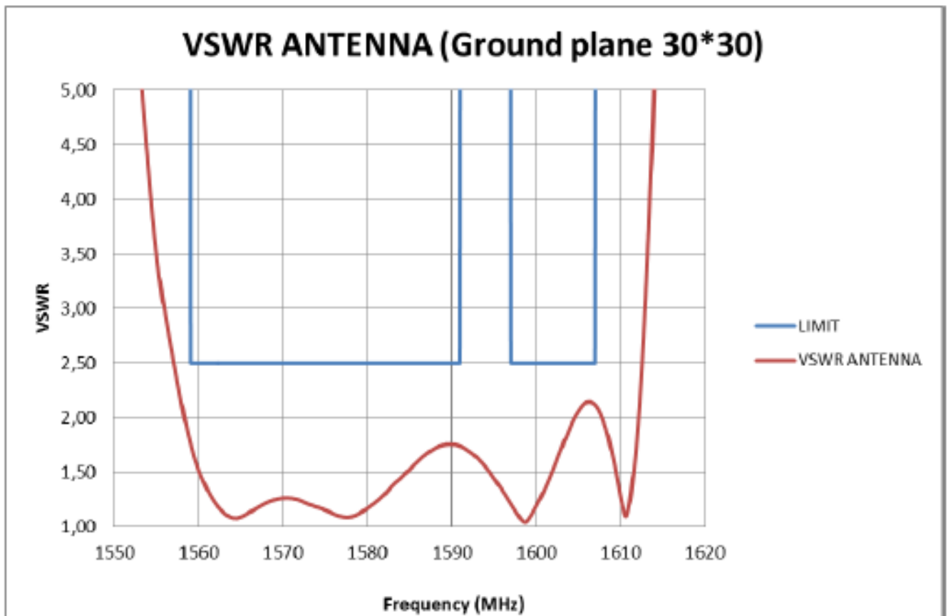
Figure 1: VSWR
