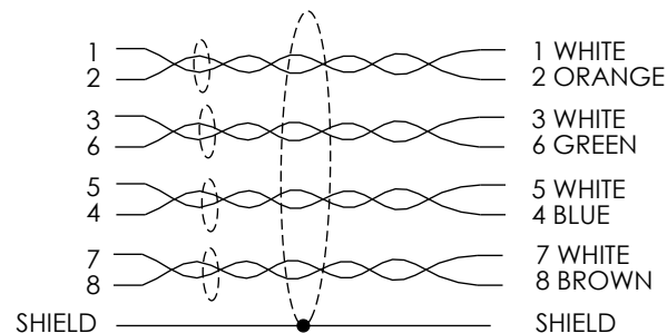
P1 WIRING MAP
