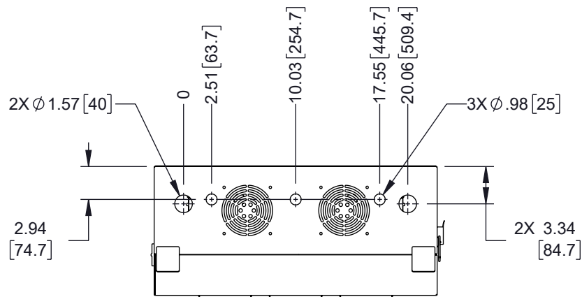
VIEW C-C
