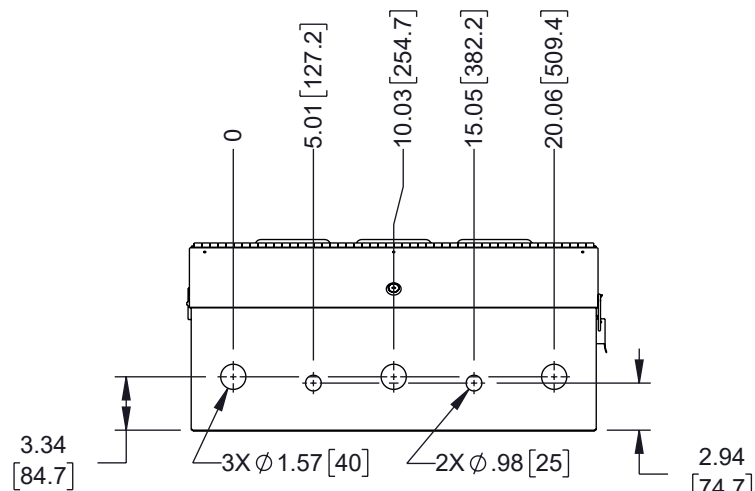
VIEW B-B
