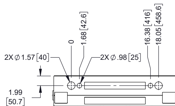
VIEW C-C
