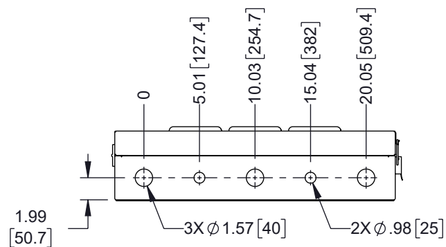
VIEW B-B
