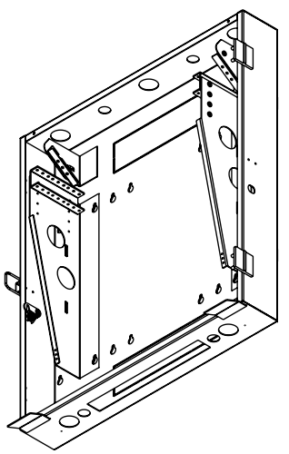
VIEW A-A POPULATED ENCLOSURE DOOR NOT SHOWN
