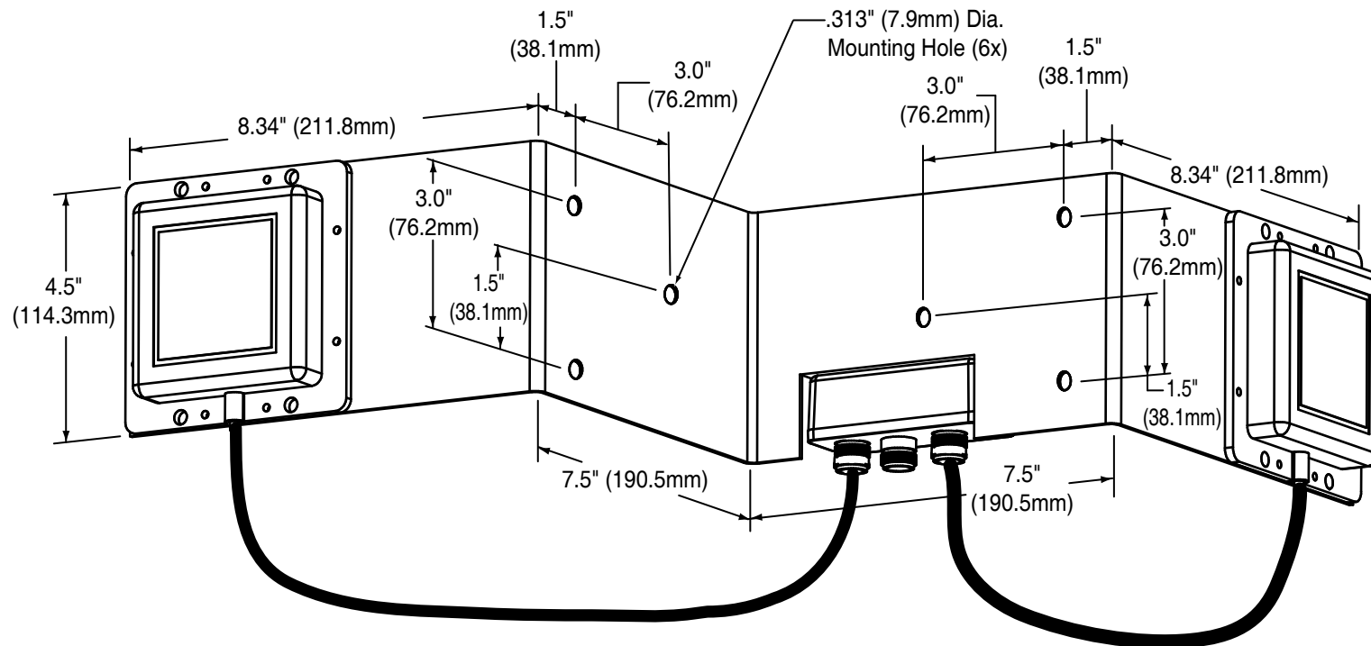
Shown with 8 dBi Antennas (HG2409P, HG5308P or HG5808P) and Splitter
