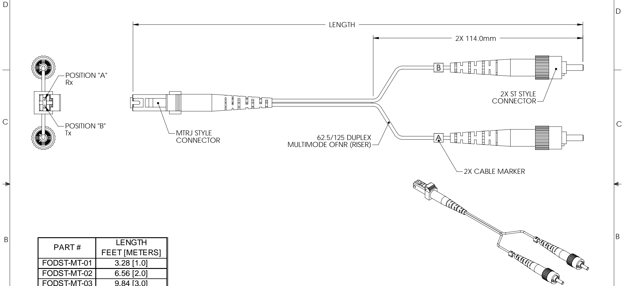
OUTLINE DRAWING
