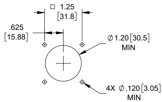
RECOMMENDED MTG HOLE PATTERN
