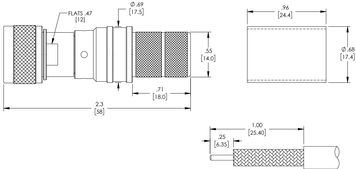
RECOMMENDED CABLE STRIPPING DIMENSIONS
