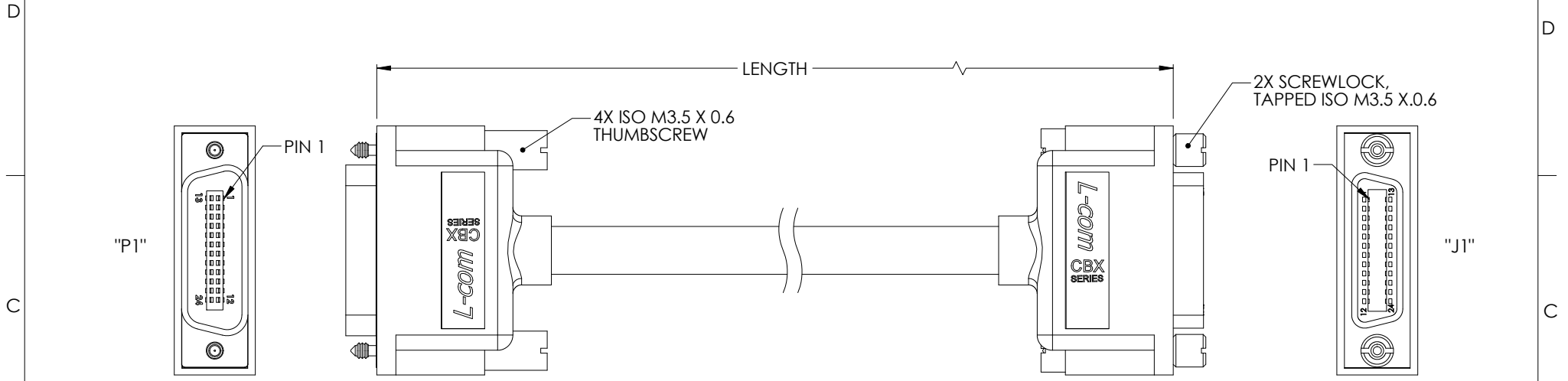
MALE, 24-PIN GPIB RIBBON CABLE
