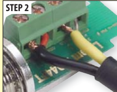
Insert center conductors, shields and tighten set screws.
