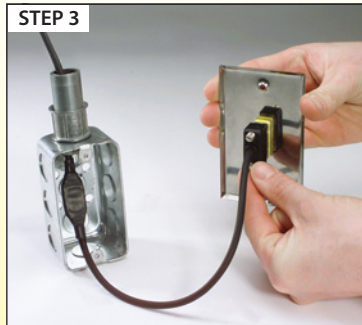
Attach pre-terminated HD15 connector to faceplate and attach to outlet.
