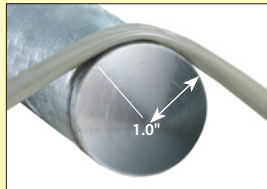
The minimum recommended bend radius for UTP is 1.0".
